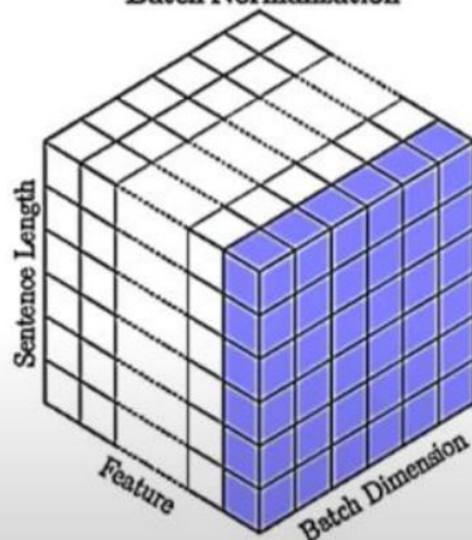
Batch Normalization
