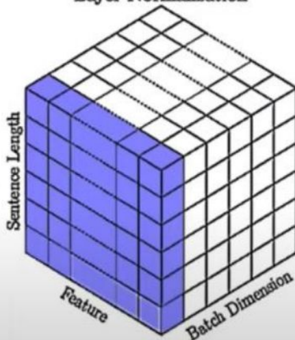
Layer Normalization
